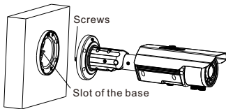
Figure 3-1 Installing camera
