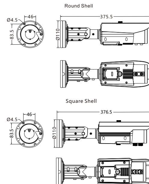
Figure 2-3 Dimensions ( Unit:mm )
