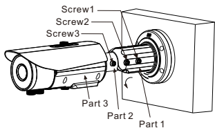
Figure 3-3 Loosening screws
